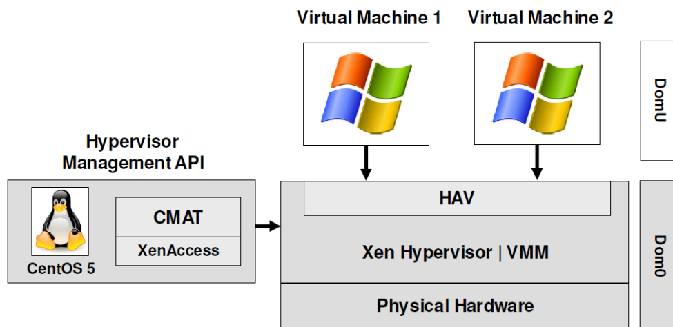
Figure 2.2: CMAT-V Architecture [47].
